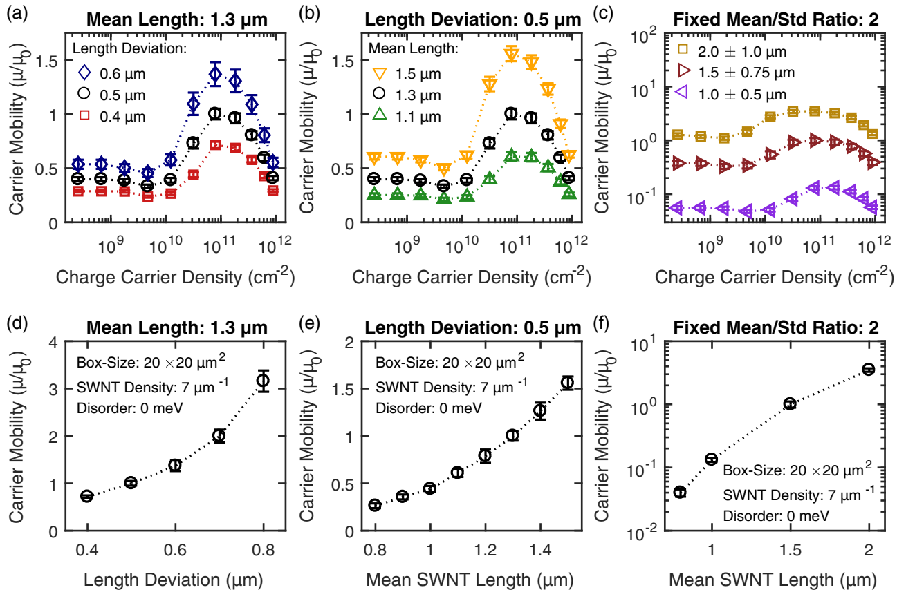
FIG. 7. Normalized carrier mobilities for different SWNT length distributions (no energetic disorder, SWNT density 7 \mu\text{m}^{-1} , simulation box size 20 \times 20 \mu\text{m}^2 ). Mobility versus charge carrier density and peak mobility versus length standard deviation for fixed SWNT mean length of 1.3 \mu\text{m} (a),(d), mobility versus charge carrier density and peak mobility versus mean SWNT length for fixed SWNT length standard deviation of 0.5 \mu\text{m} (b),(e), and for fixed ratio between the mean length and length standard deviation of 2 (c),(f). Dotted lines are guides to the eye.
