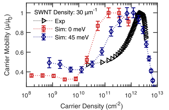
FIG. 10. Experimental [52] and simulated normalized mobility versus charge carrier density for (6,5) SWNT networks. Simulated results are given for the cases without energetic disorder and an energy disorder of 45 meV. The SWNT density was estimated from the experiments to be 30 \mu\text{m}^{-1} . Dotted lines are guides to the eye.
