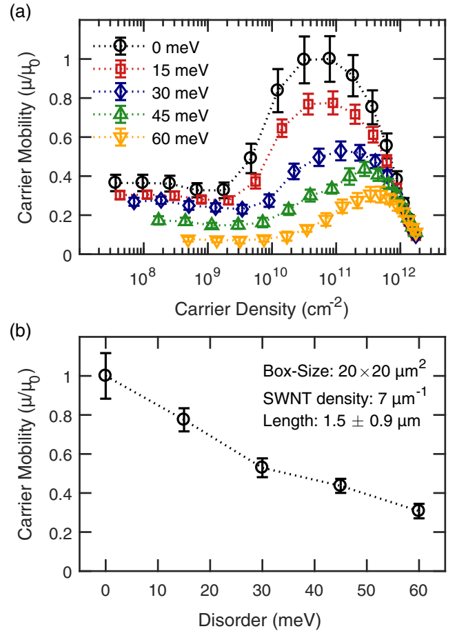
FIG. 4. Network mobilities for different disorder strengths (simulation box size: 20 \times 20 \mu\text{m}^2 , SWNT length: 1.5 \pm 0.9 \mu\text{m} , linear SWNT density: 7 \mu\text{m}^{-1} ): (a) Normalized charge carrier mobility versus carrier density. (b) Peak mobility versus disorder strength. Dotted lines are guides to the eye.
