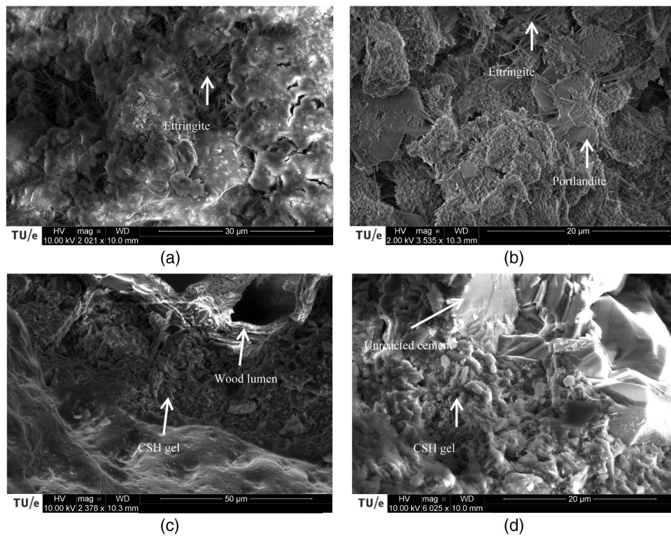
Fig. 6. SEM pictures of the microstructure of (a and b) B4 and (c and d) B1 around wood-wool
