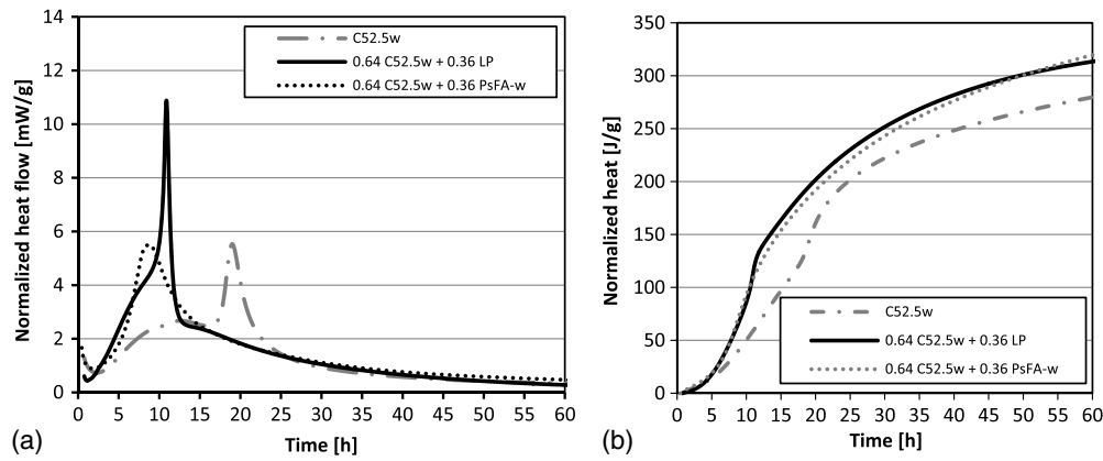
Fig. 3. (a) Normalized heat flow and (b) normalized heat of mixtures consist of C52.5w compared to 0.64 C52.5w + 0.36PsFA-w and 0.64C52.5w + 0.36LP; mixtures are produced with a water-to-powder ratio of 0.5 and measured up to 60 h
