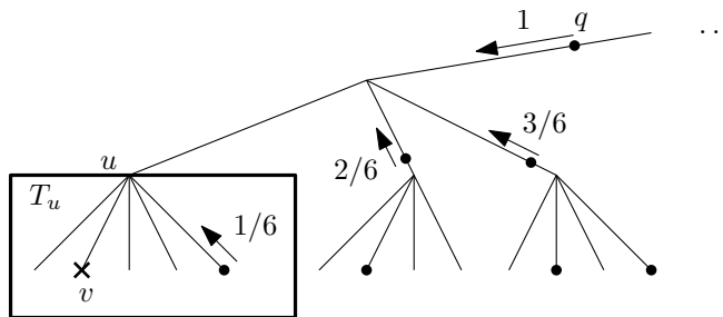
Figure 2: A request at v inside of the elementary tree T_u , and Phase 2 of Algorithm 1. Note that k_q^- equals 6 in the visualised case. Speed is noted next to each server moving.
