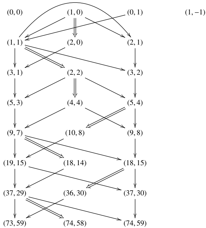
Figure 4.3 A uniform add-double-add two-dimensional ladder.
