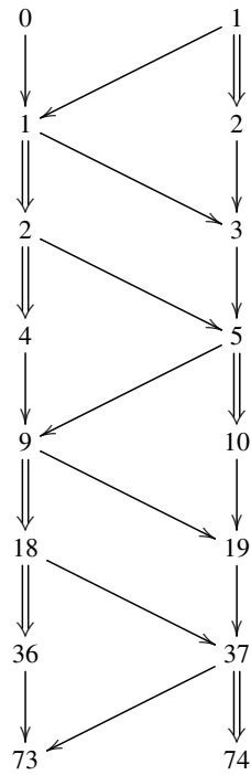
Figure 4.1 A uniform double-add ladder.
