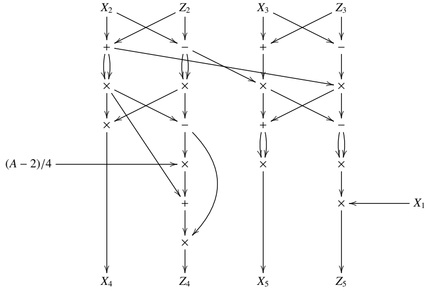
Figure 4.2 Montgomery's optimized formulas for doubling and differential addition, assuming Z_1 = 1 .
