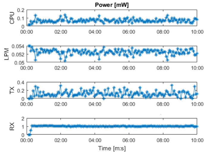
FIGURE 4.4: Power consumption analysis of the PAN coordinator in the TSCH example (X axis represents time in minutes:seconds, Y axis represents the power consumed in mW by the Z1 mote for CPU, LPM (low power mode/idle), Tx and Rx)
