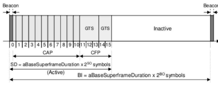
FIGURE 2.6: IEEE 802.15.4 superframe structure [6].
