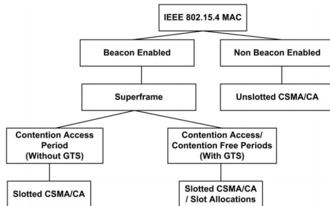
FIGURE 2.5: IEEE 802.15.4 operation modes [3].
