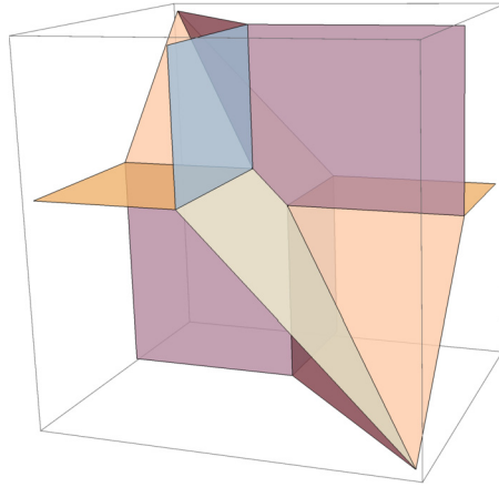
Fig. 1. The cell decomposition for a matroid flock; the two zero-dimensional cells are 0 and -ge_2 - ge_3 .
