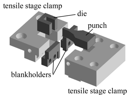
Figure 1: Exploded view of the experimental deep-draw setup.
