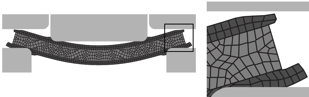
Figure 4: Result of a simulation (left) where the delaminated areas are clearly visible (right).
