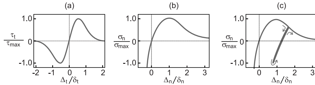
Figure 3: (a) The reversible cohesive law from eqn (1) in tangential direction and (b) from eqn (2) in normal direction, with \tau_{max} as maximum shear stress and \sigma_{max} as the maximum normal stress. (c) The irreversible cohesive law in normal direction.
