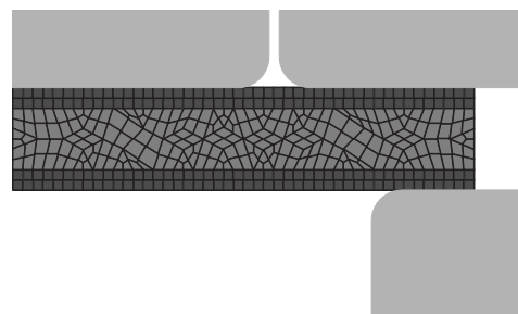
Figure 2: The plane strain model geometry of the experimental deep-draw setup with a polymer coated ECCS strip. Due to symmetry, only half the geometry is modelled.
